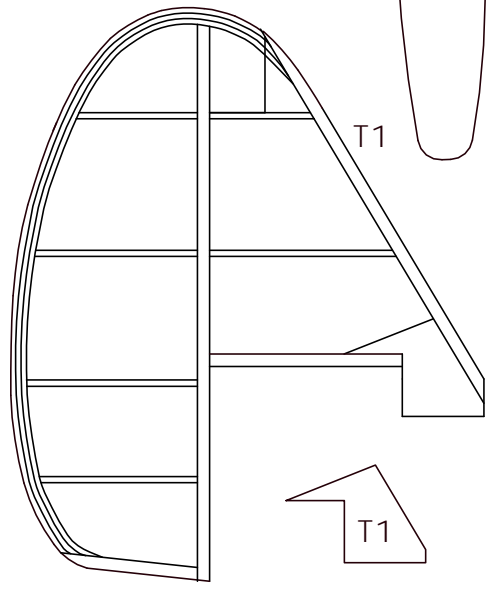
Wing tip laminating template
